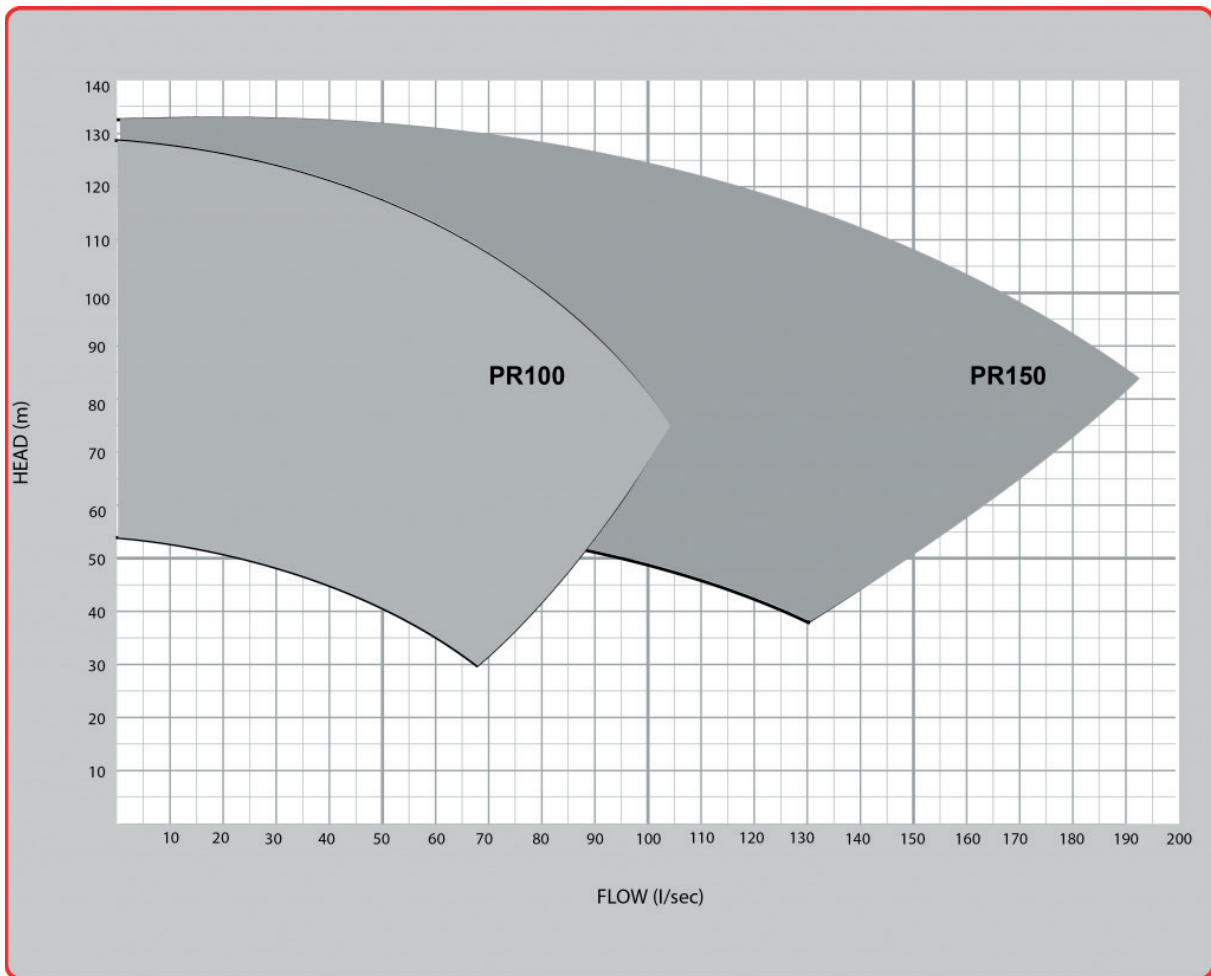
Coverage Chart for Battlemax PR Pumps
