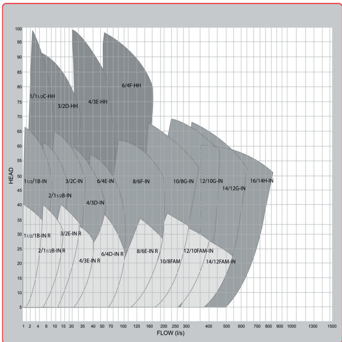
Coverage chart for international series pumps
