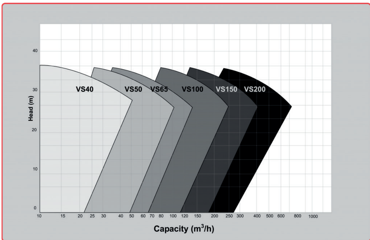
Coverage Chart for Battlemax Vertical Spindle Slurry Pumps
