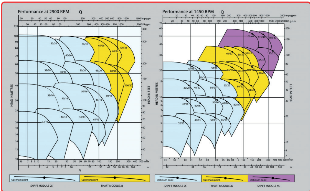
Coverage Chart for Battlestream
