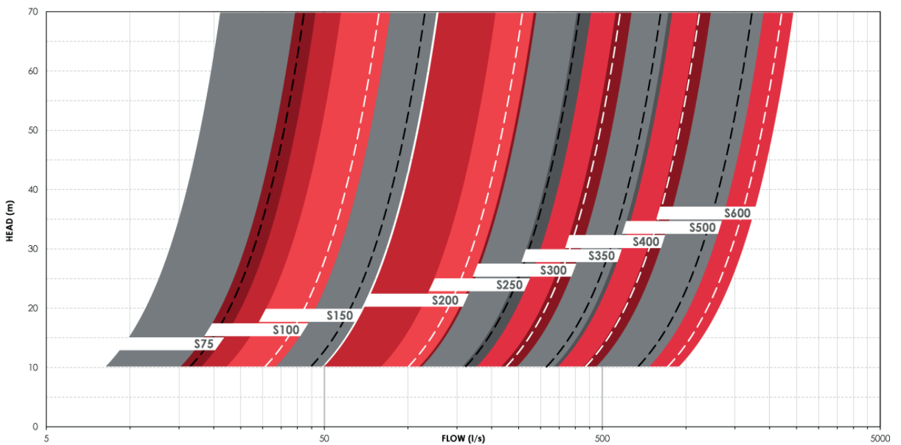
Flow Coverage Map Per S-Range Pump Model: 0.5 \cdot Q_{bep} - 1.1 \cdot Q_{bep}
