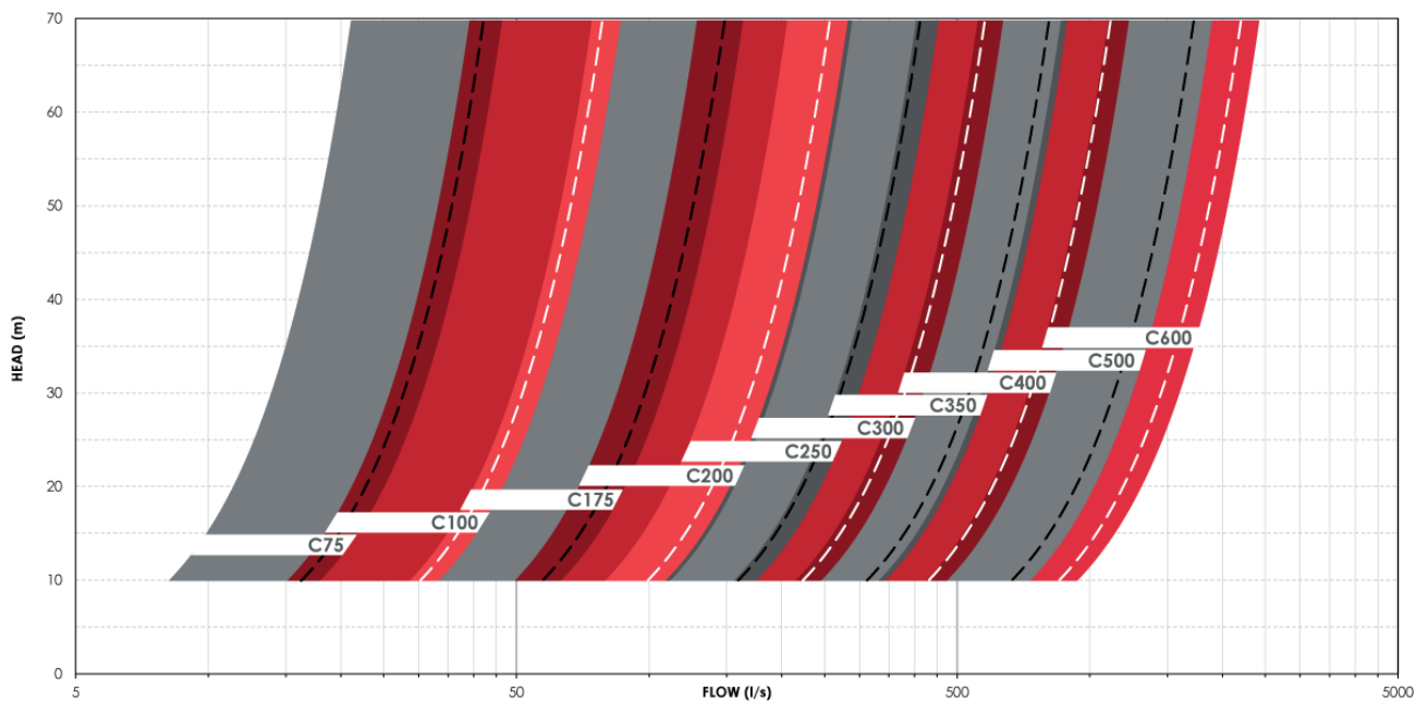
Flow Coverage Map Per C-Range Pump Model: 0.5 \cdot Q_{bep} - 1.1 \cdot Q_{bep}
