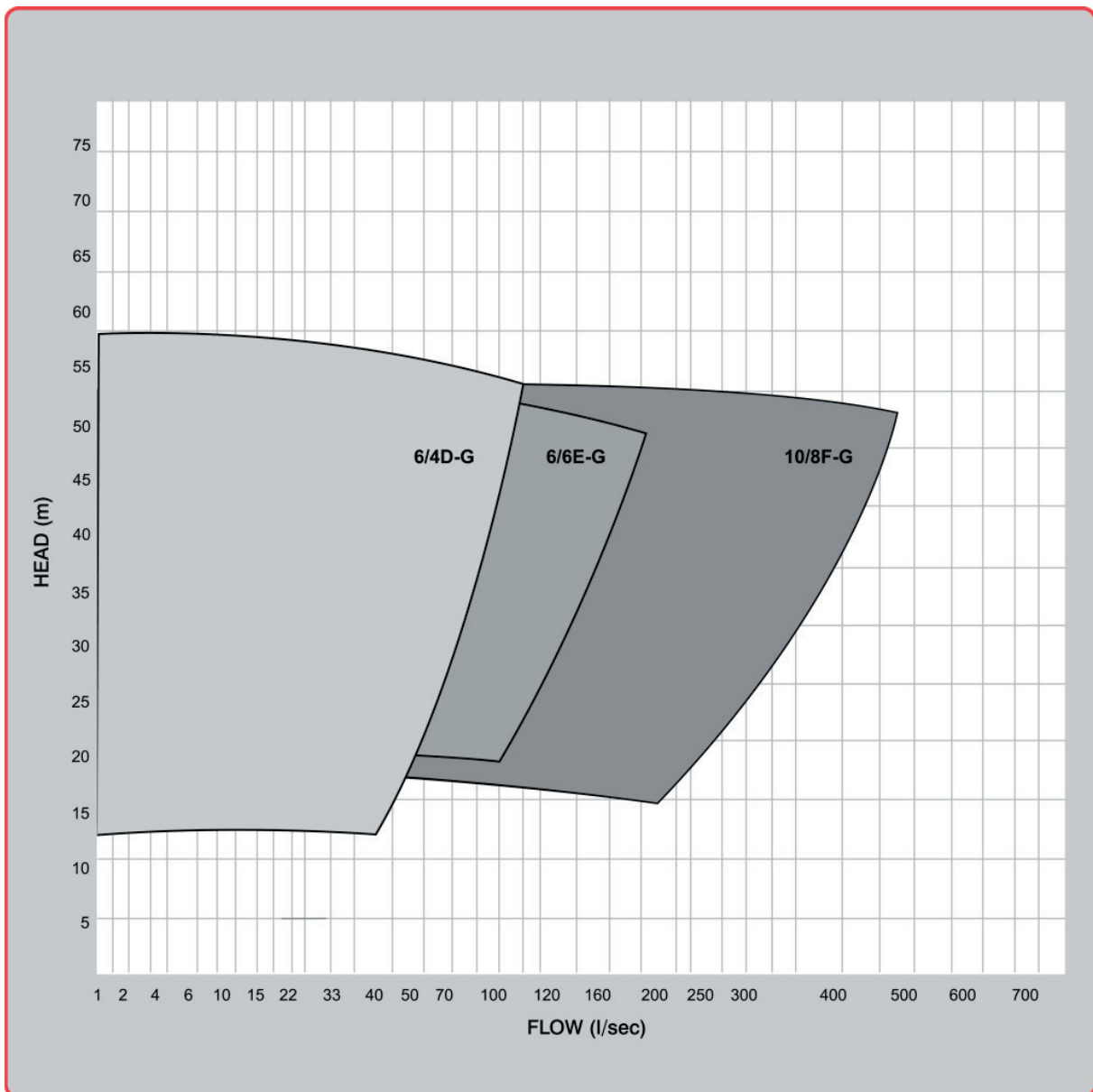
Coverage Chart for Battlemax Gravel Slurry Pumps
