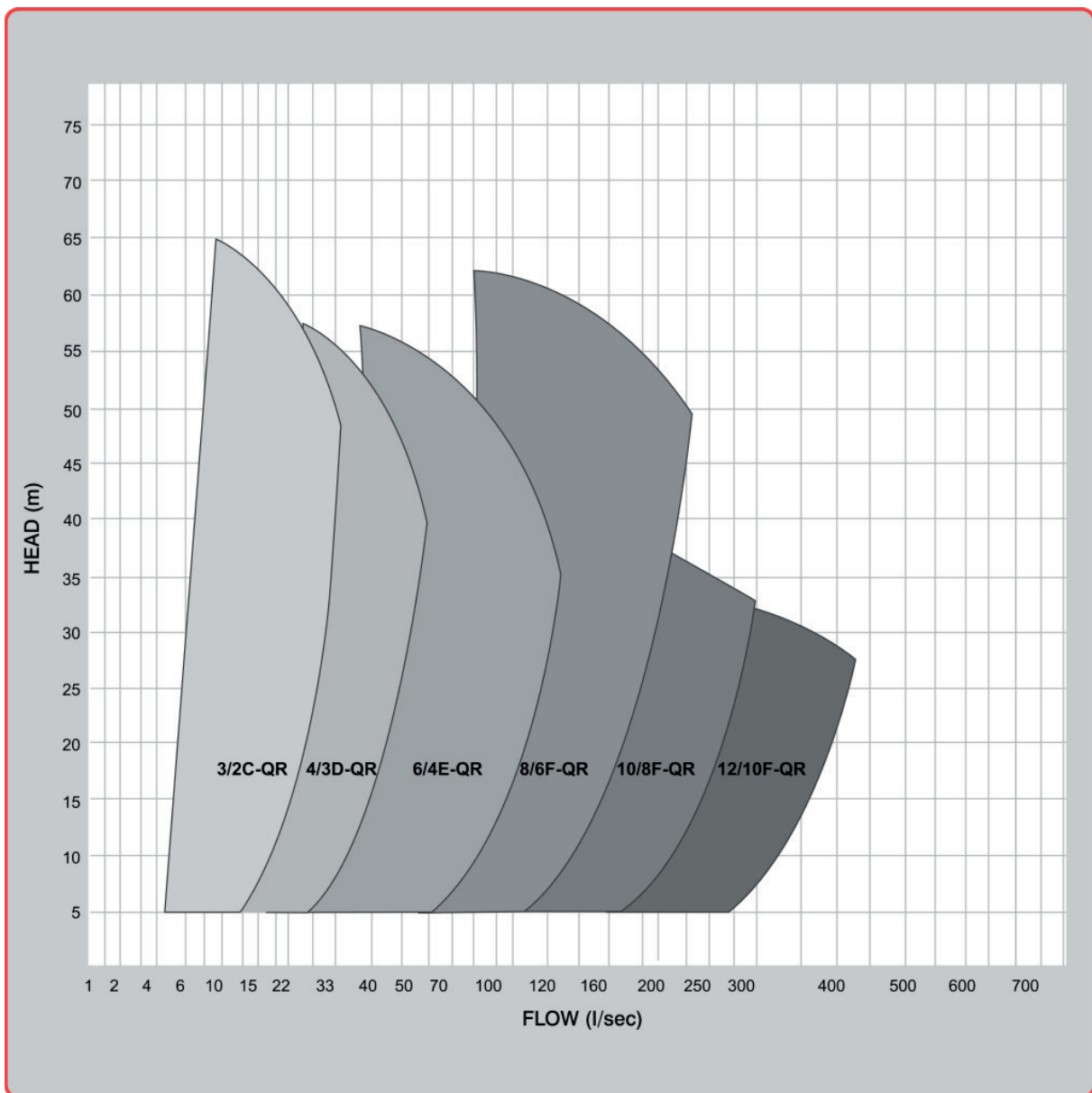
Coverage Chart for Battlemax Quick Release Pumps
